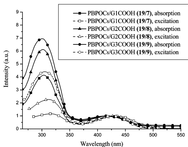
Figure 8. UV-vis absorption and corrected excitation spectra of symmetric H-bonded dendrimers (with different generations of donor dendrimers) PBP-OC 8 /G1COOH ( 19/7 ), PBP-OC 8 /G2COOH ( 19/8 ), and PBP-OC 8 /G3COOH ( 19/9 ) monitored at the core of double H-bonded acceptor emitter PBP-OC 8 ( 19 ).
