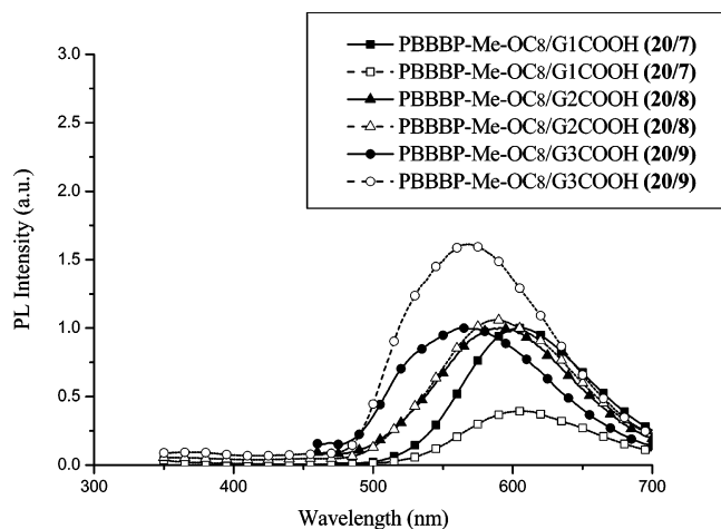
Figure 12. PL spectra of symmetric supramolecular dendrimers containing double H-bonded acceptor emitter PBBBP-Me-OC 8 ( 20 ) in thin films as they were excited at the maximum absorption of the dendritic peripheral OXD units (at 305 nm for open symbols) and at the maximum absorption of the emitting core PBBBP-Me-OC 8 ( 20 ) in H-bonded G1-G3 dendrimers (at 450, 446, 439 nm, respectively, for solid symbols).
