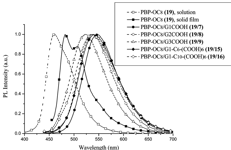
Figure 6. Normalized PL spectra of bis-pyridyl (double H-bonded) acceptor emitter PBP-OC 8 ( 19 ) and its H-bonded dendrimers.
