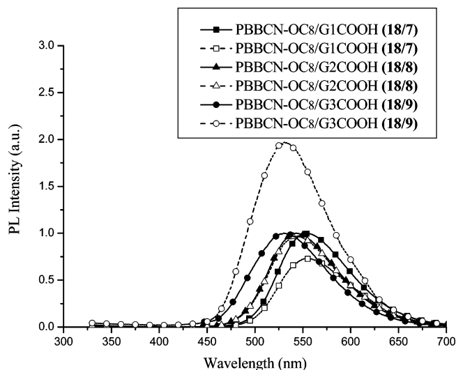
Figure 10. PL spectra of asymmetric supramolecular dendrimers containing single H-bonded acceptor emitter PBBCN-OC 8 ( 18 ) in thin films, which were excited at the dendritic peripheral OXD units (at 305 nm for open symbols) and at the maximum absorption of the emitting core PBBCN-OC 8 ( 18 ) in H-bonded G1–G3 dendrimers (at 424, 423, and 419 nm, respectively, for solid symbols).
