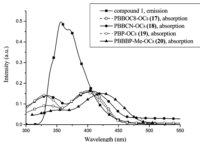
Figure 7. UV-vis absorption spectra of (single/double H-bonded) acceptor emitters PBBOC 8 -OC 8 ( 17 ), PBBCN-OC 8 ( 18 ), PBP-OC 8 ( 19 ), and PBBBP-Me-OC 8 ( 20 ) and PL spectrum of compound 1 (containing an OXD unit) in THF. It indicates that an overlap exists between the emission band of the donor and the absorption bands of the acceptor emitters, resulting in energy transfer from OXD units to the emitting core.
