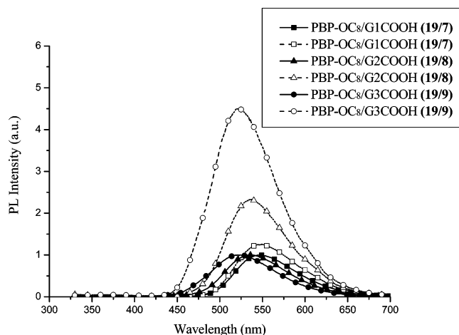
Figure 9. PL spectra of symmetric supramolecular dendrimers containing double H-bonded acceptor emitter PBP-OC 8 ( 19 ) in thin films, which were excited at the dendritic peripheral OXD units (at 305 nm for open symbols) and at the maximum absorption of the emitting core PBP-OC 8 ( 19 ) in H-bonded G1–G3 dendrimers (at 418, 415, 408 nm, respectively, for solid symbols).
